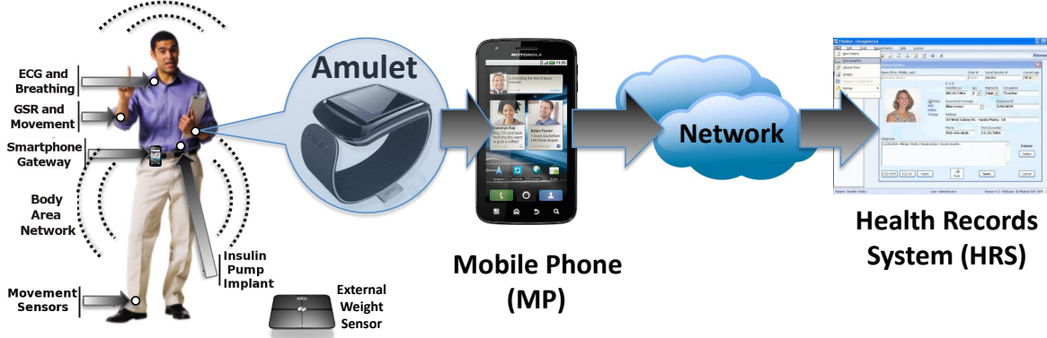
Figure 1: Our proposed architecture is built around a trustworthy wrist-worn Amulet device.
