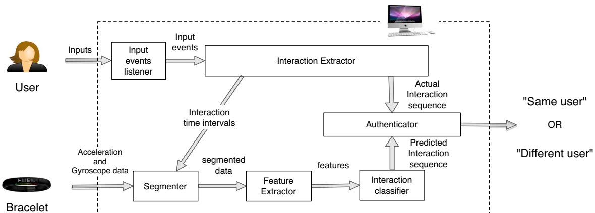
Figure 2: ZEBRA architecture.
